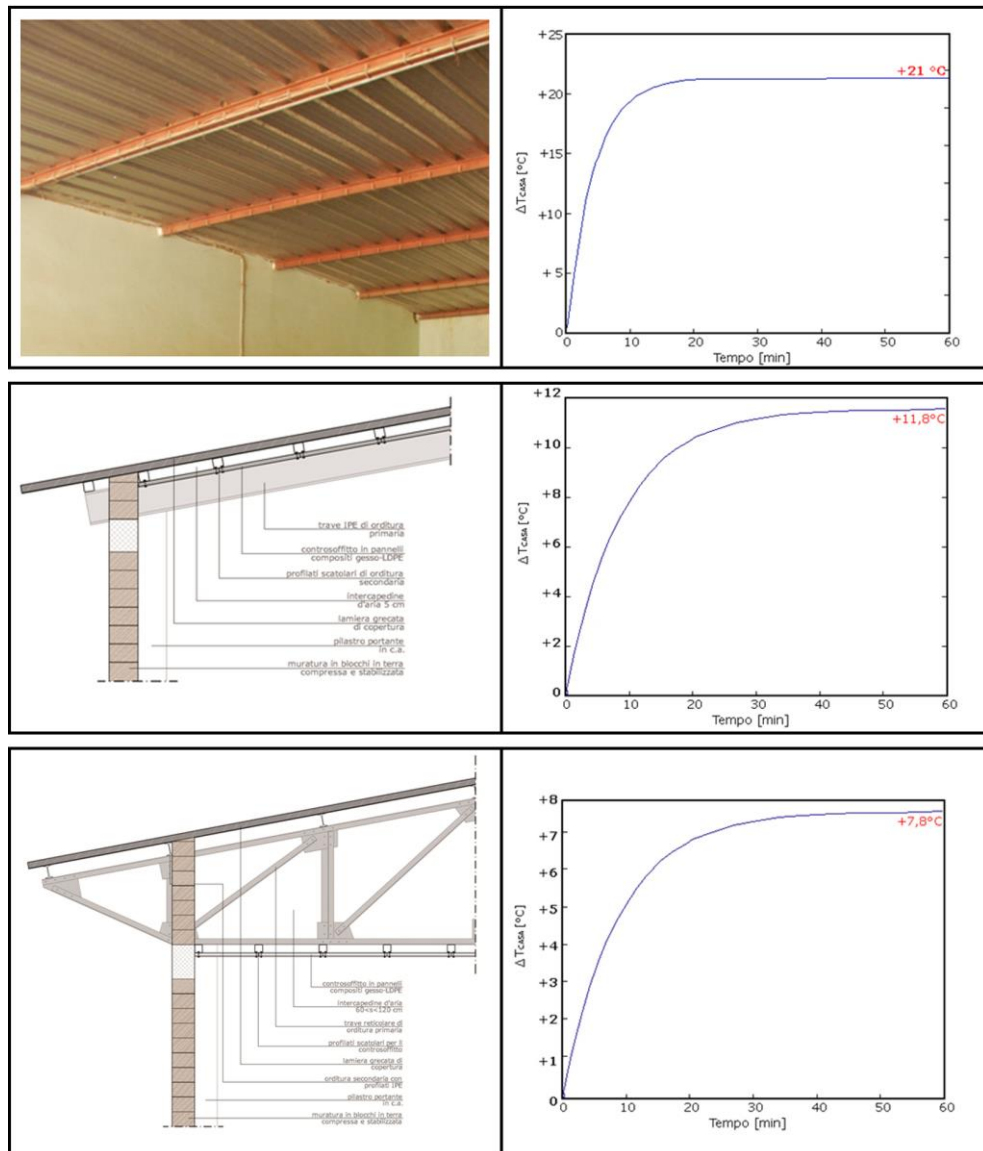
Figure 5: Three scenarios: scheme + inside temperature simulation.
