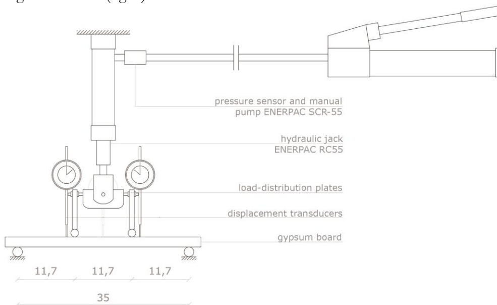
Figure 2. Bending test - instruments scheme
